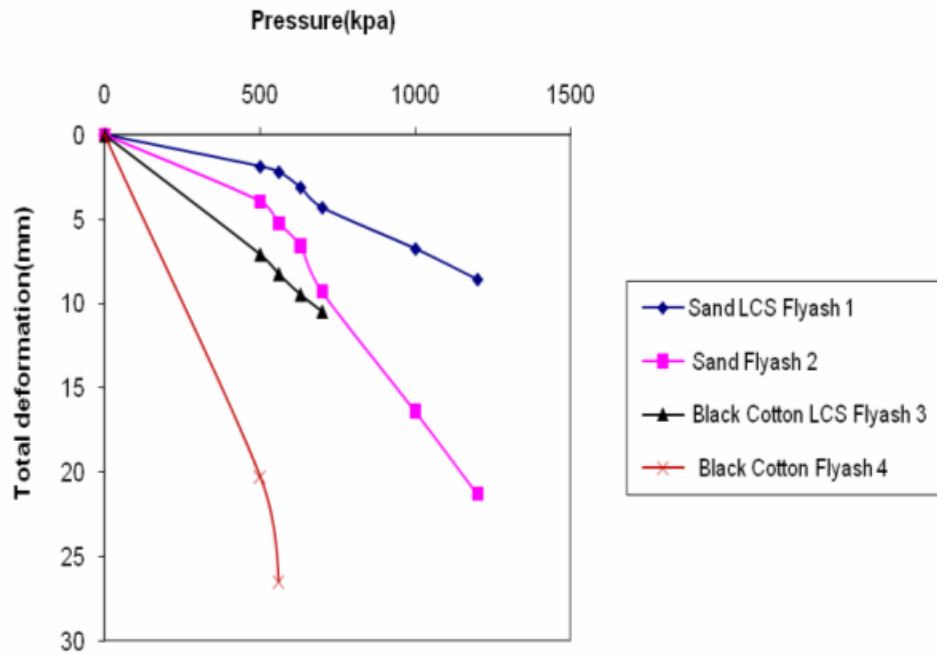
Figure-4. Pressure total deformation curves of all the stretches on different subgrades in the field.
