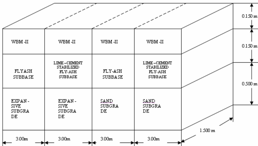
Figure-1. Flexible pavement test tracks on different subgrades.
