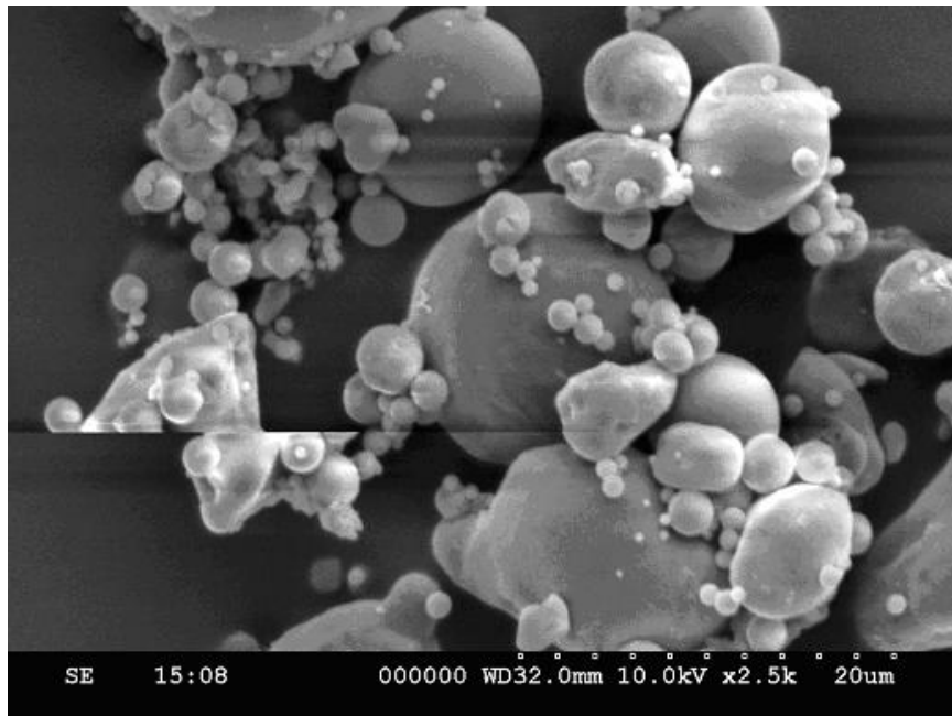
Figure-5. Scanning electron micrograph (SEM) for untreated flyash.
