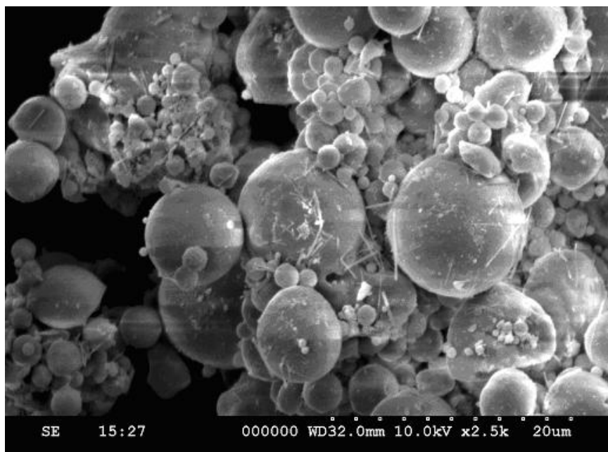
Figure-6. SEM for flyash treated with 2% of lime + 0.5% of cement.
