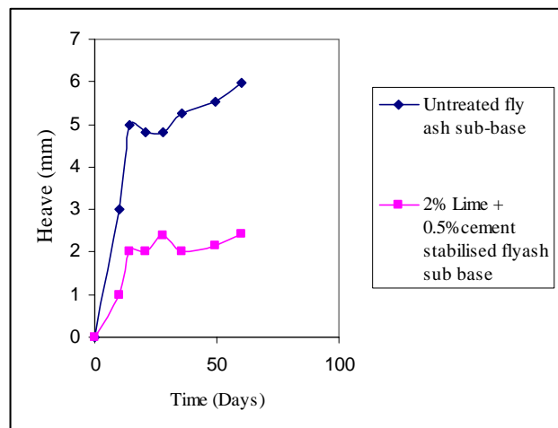
Figure-3. Heave-time plots for different tracks laid on expansive soil subgrade in the field.
