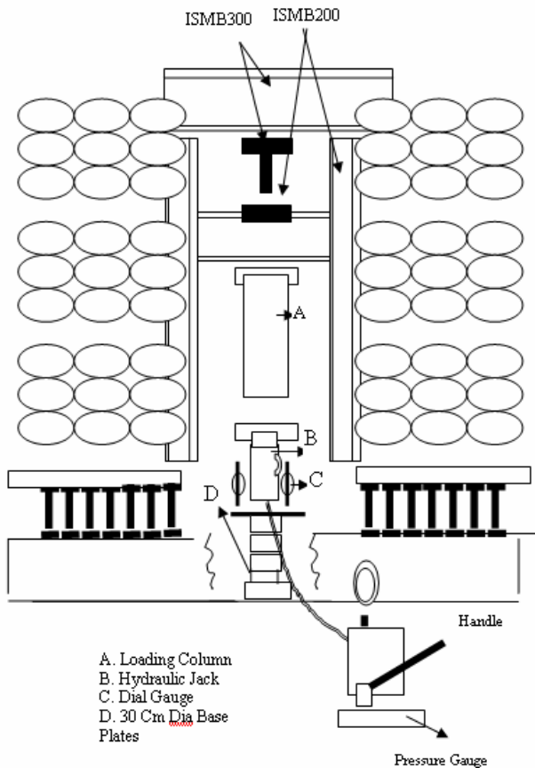
Figure-2. Schematic diagram of plate load test setup.
