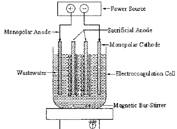
Figure-3. Bench-scale EC reactor with bipolar electrodes in parallel connection (after [23]).
