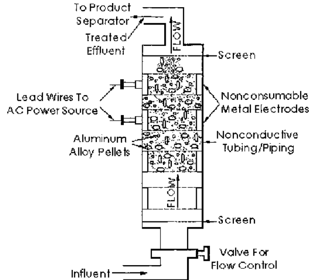
Figure-4. Flow diagram of a typical ACE fluidized separator (based on Recra Environmental Inc., USA).
