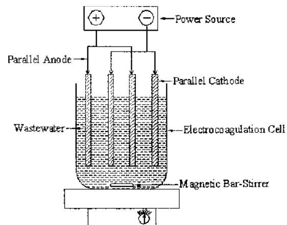
Figure-1. Bench-scale EC reactor with monopolar electrodes in parallel connection (after [23]).
