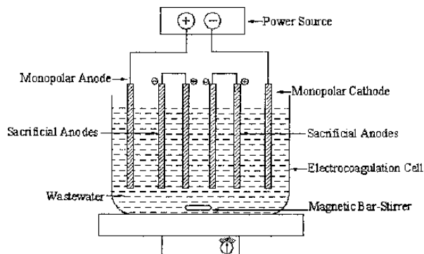
Figure-2. Bench-scale EC reactor with monopolar electrodes in series connection (after [23]).
