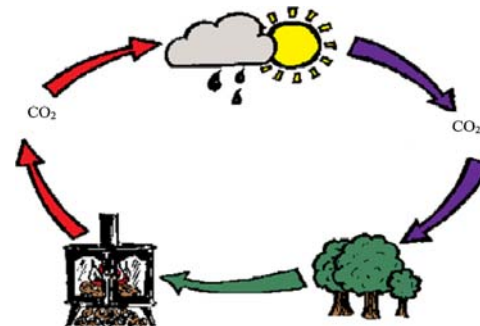
Figure-2. Carbon Cycle.
