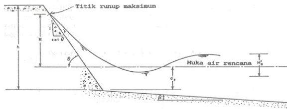
Figure-2. Wave Run-Up.
