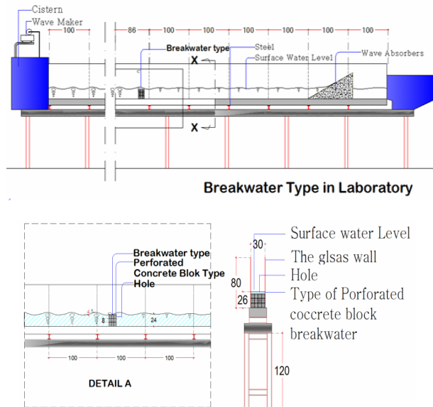
Figure-2. Model of Breakwater Simulation
