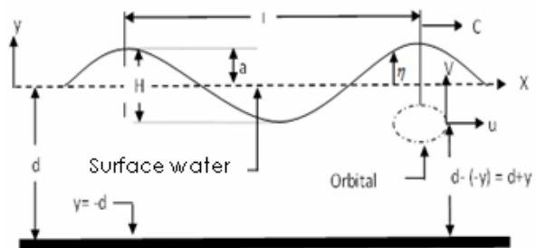
Figure-1. Wave Airy Theory.
