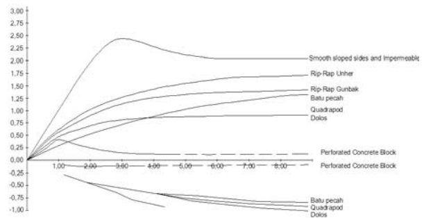
Figure-5. Graph of comparison of the run-up based on the material making up the breakwater.
