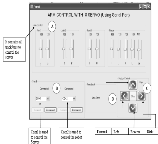
Figure-3. Window form application for GUI interface
