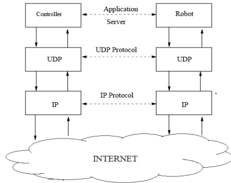
Figure-4. Layers of control network.
