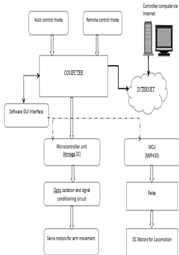
Figure-7. Basic function block diagram.
