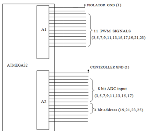
Figure-2. Connection diagram with Atmega32.
