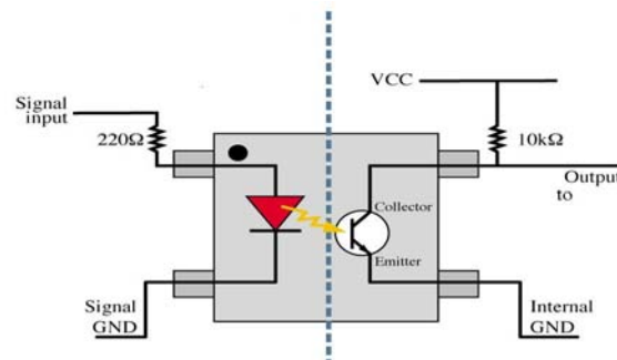
Figure-5. Opto coupler Isolation circuit diagram.
