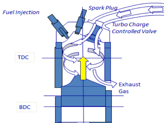
Figure-1. Turbo charge cleaning combustion chamber.
