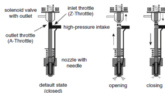
Figure-2. Servo injector and nozzle design.
