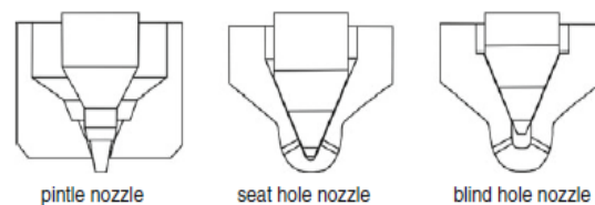
Figure-3. Injector nozzle design.
