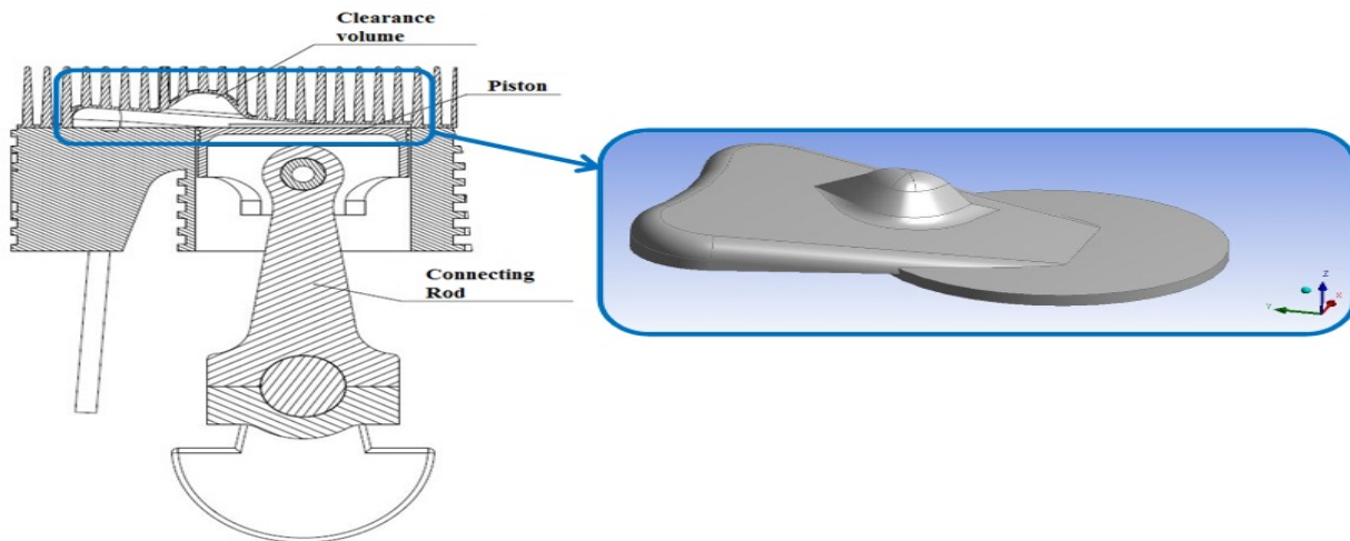
Figure-1. Clearance volume of the in-cylinder engine and imported domain in ANSYS workbench.
