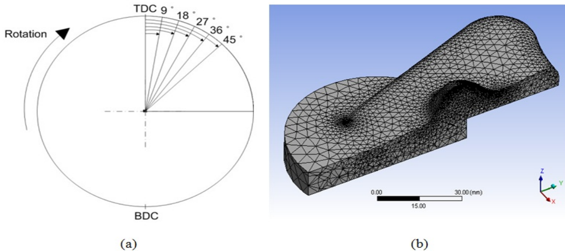
Figure-2. (a) Complete cycle; (b) Cut-view of the clearance volume of the engine.
