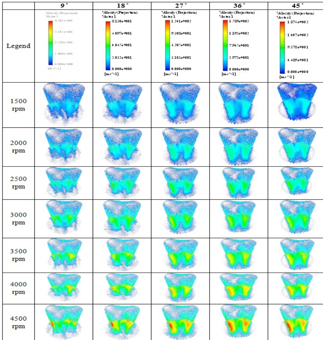
Figure-3. Flow viewed from Plane A.
