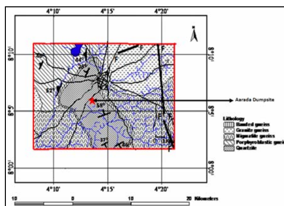
Figure-1b. Geologic Map of Ogbomoso (modified after Afolabi et al., 2011).
