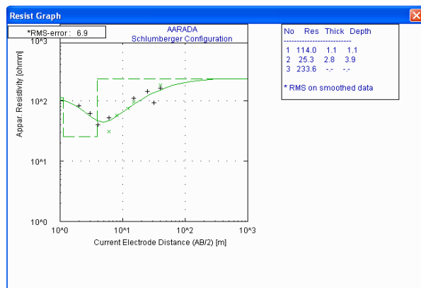
Figure-7. Modeled curve for VES-5.
