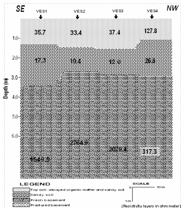
Figure-10. Geoelectric section beneath VES 1, 2, 3 and 4.
